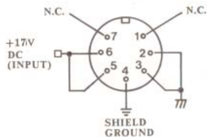
Figure C-1 Power connector
